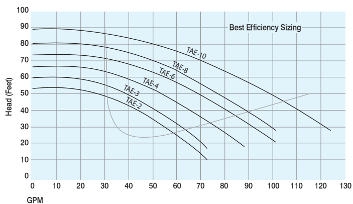
60HZ Performance
