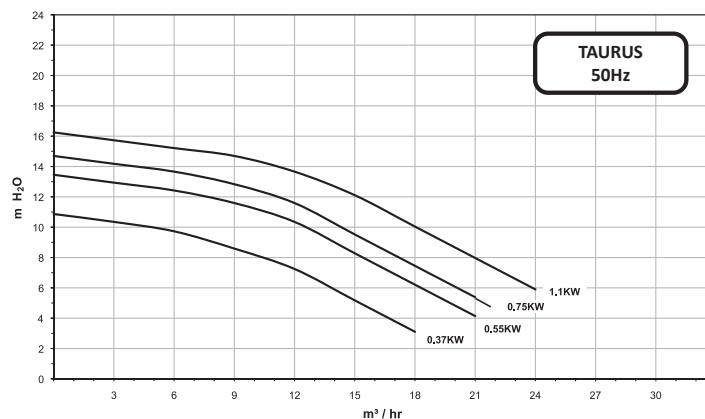
50HZ Performance
